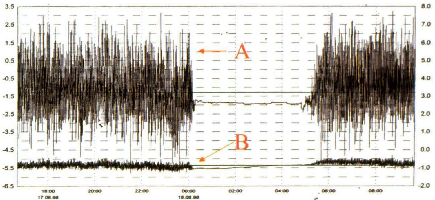
Comparing P/S potential(A) with polarization potential(B) measured with polarization potential probe at the area beneath subway stray current
